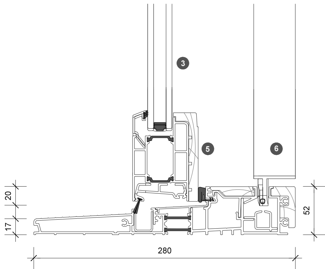
4. sill detail
